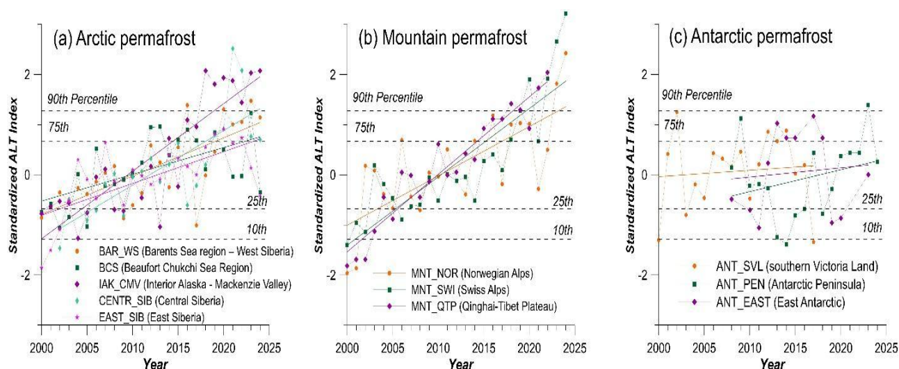
Figure 1. Standardized index of active layer thickness (ALT) relative to 2000–2020 baseline. (a) Arctic regions: Beaufort Chukchi Sea – Arctic Alaska and Mackenzie Delta region (BCS), Interior Alaska and central Mackenzie Valley, Northwest Territories (IAK_CMV), Barents Sea region – West Siberia (BAR_WS), Central Siberia (CENTR_SIB), East Siberia (EAST_SIB); (b) Mountain regions: Norwegian mountains (MNT_NOR), Swiss Alps (MNT_SWI), Qinghai-Tibet Plateau (MNT_QTP); and (c) Antarctic: southern Victoria Land (ANT_SVL), Antarctic Peninsula (ANT_PEN), East Antarctic (ANT_EAST).
