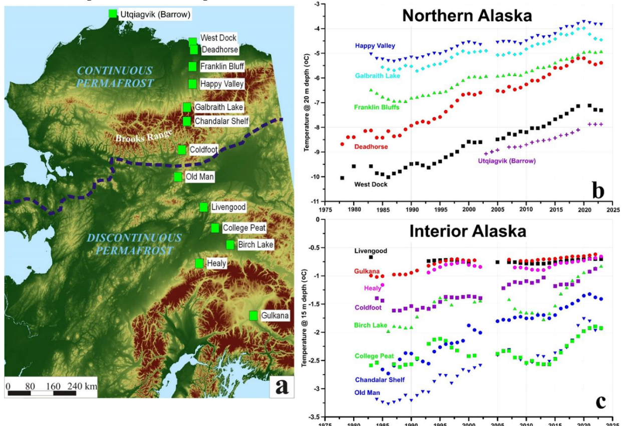
Fig. 1. Continuous and discontinuous permafrost zones in Alaska (separated by the broken blue line) and location of a north-south transect of permafrost temperature measurement sites (a); time series of mean annual temperature at depths of 20 m (b) and 15 m (c) below the surface, respectively, at the measurement sites.
